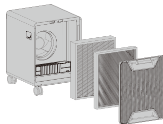
Remove Filters and UV (AG600/900 Model)
